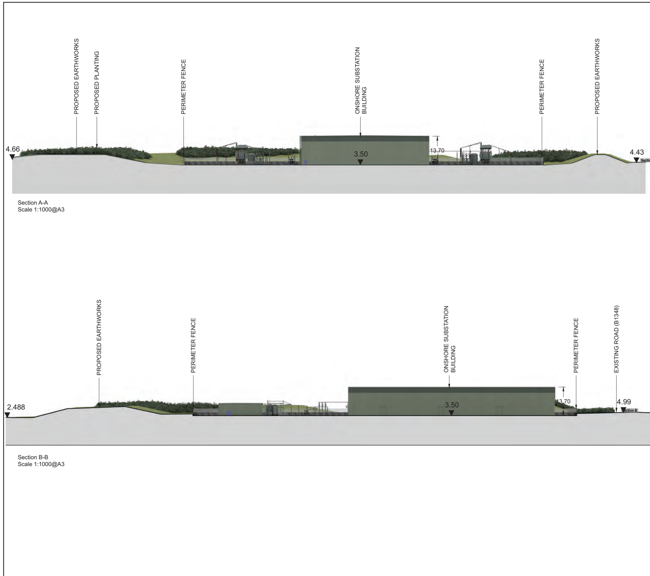
Fig 8.6b Landscape Mitigation Cross Sections
